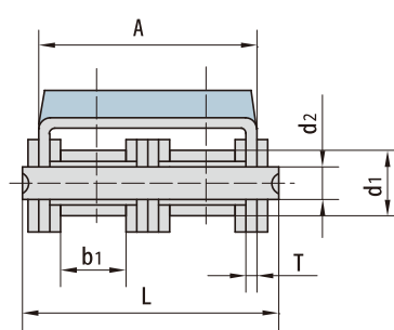
带G 2部件 With G 2 profile
